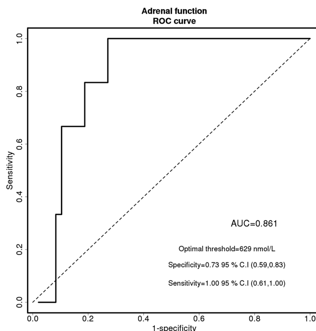
Figure 7 The ROC curve for logistic regression model that uses stimulated cortisol level at visit 1 as the explanatory variable for developing adrenal insufficiency after the 30-day MPSL treatment protocol.
