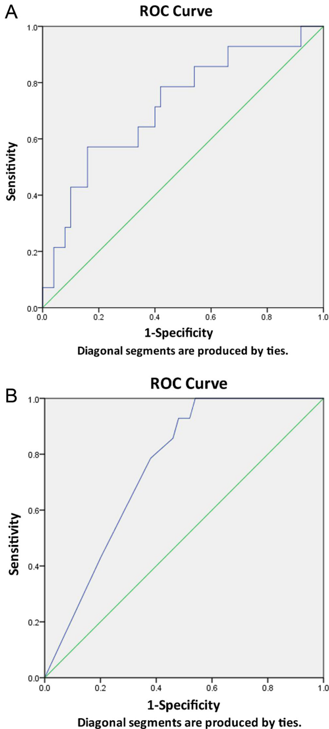
Figure 1 ROC curve analysis of CRP and TSH levels to identify a cutoff level for hypothyroidism. (A) The cutoff level for CRP was found to be 97.80 mg/L (AUC: 0.717, P : 0.014; sensitivity: 57.1%; specificity: 84.0%) and (B) the cutoff level for TSH was found to be 0.10 mIU/L (AUC: 0.752, P : 0.004; sensitivity: 100%; specificity: 46.0%).
